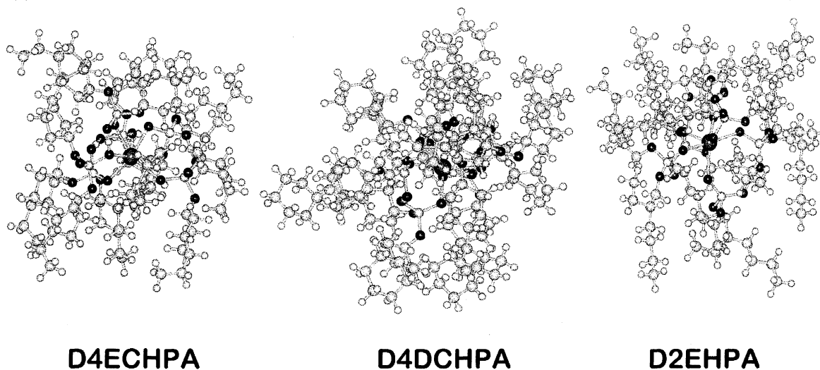
Fig. 7. (a) Proposed structures of rare earth complexes with D4ECHPA, D4DCHPA and D2EHPA. (b) Proposed ball and stick model structures of \text{Sm}^{\text{III}} complexes with D4ECHPA, D4DCHPA, and D2EHPA calculated by molecular mechanics method, MOMECC.
